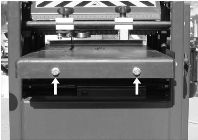
On the inner side of the table edge there is an iron angle. When this is shifted to the outside, it serves as support and mount for your home-made feed tables. Make sure that they are at the same level as the planing table.
