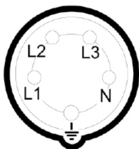
(6) Branchement 400 V
