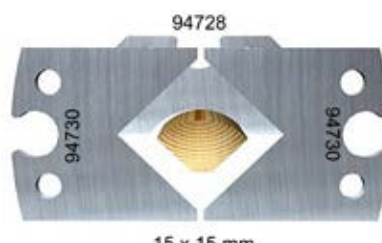
Quarter-round moulding, 15 mm
