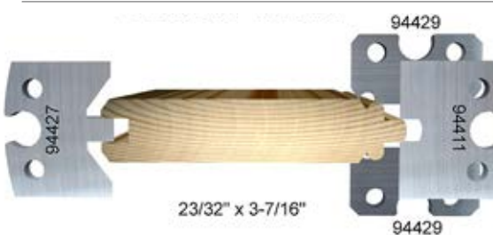
Beaded partition
