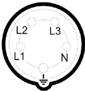
(6) Connection 400 V
