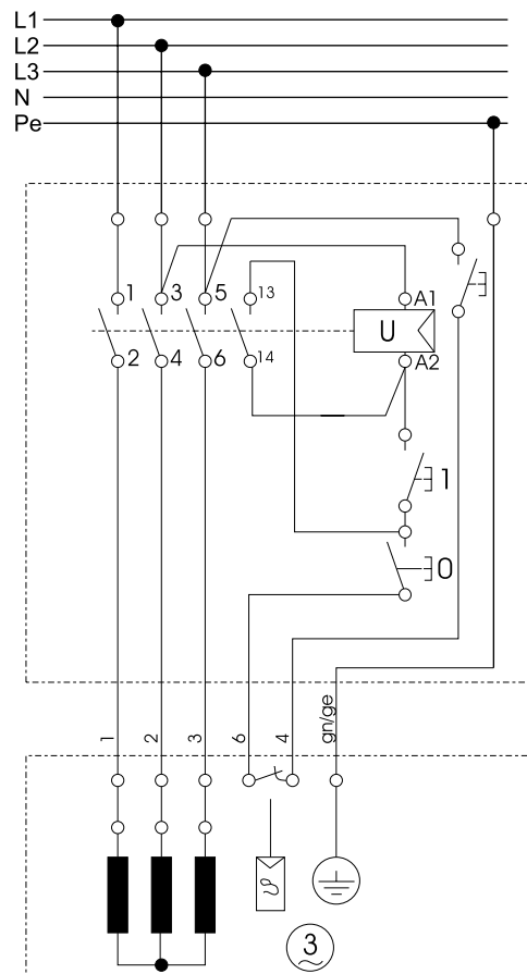
(7) Circuit diagram
