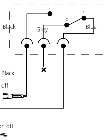
Interlock safety switch
