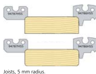
Joists, 5 mm radius.
