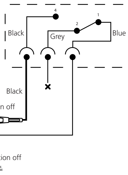
Interlock safety switch
