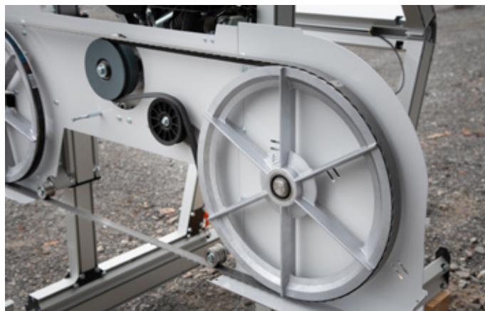
Band wheels with fan blades, cools the blade and keeps the cover clean.
