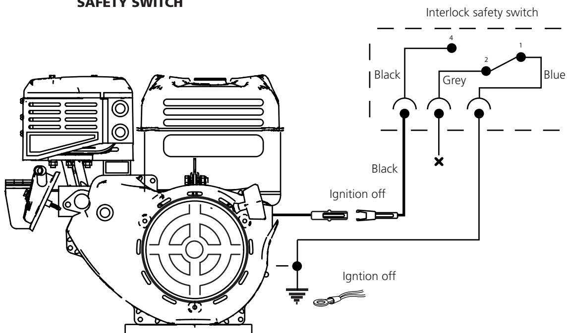
WIRING DIAGRAM, EMERGENCY STOP / SAFETY SWITCH
